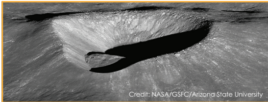
Ryder crater is located in the South Pole–Aitken Basin, which is the largest and possibly oldest basin on the Moon.
