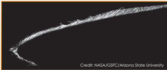
Shackleton Crater is an impact crater that lies at the lunar South Pole. While peaks along the crater's rim are exposed to almost continual sunlight, the interior is always in shadow.
