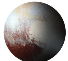
Pluto (Dwarf planet)
