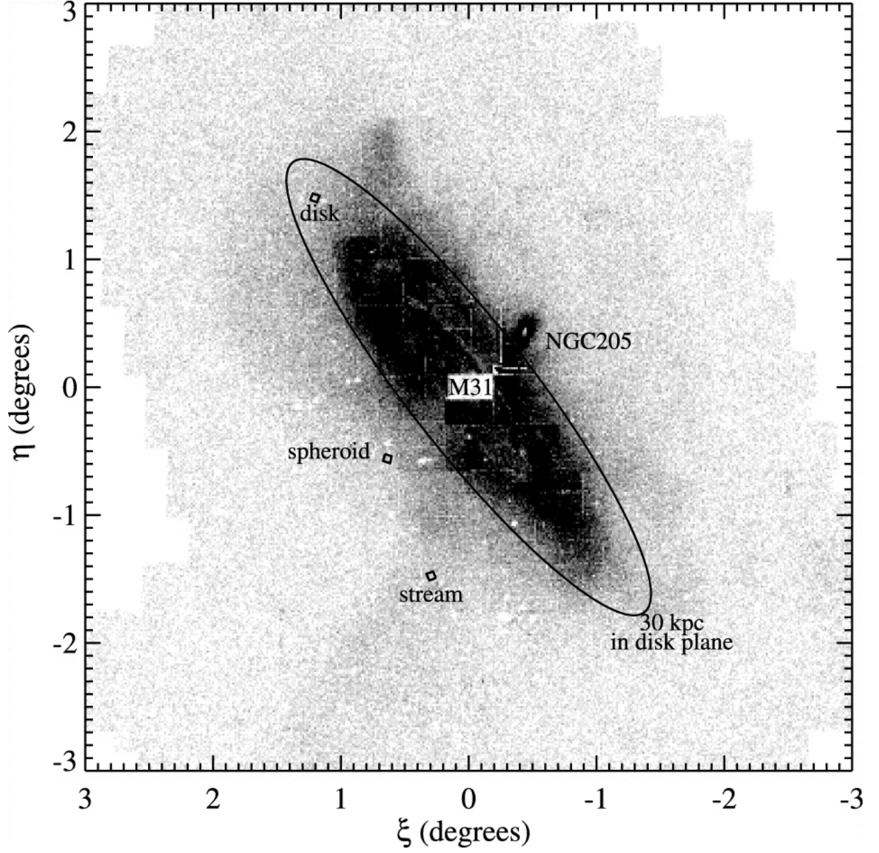
Fig. 1.— Figure taken from Brown et al. (2006). Appropriately scaled and rotated boxes denote our three target fields (labeled). The underlying gray shading represents the density of stars from the map of Ferguson et al. (2002). The ellipse marks the area within 30 kpc of the galactic center in the inclined disk plane (labeled).
